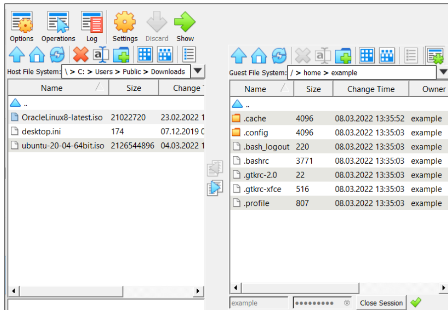
Figure 13: Guest Control File Manager
