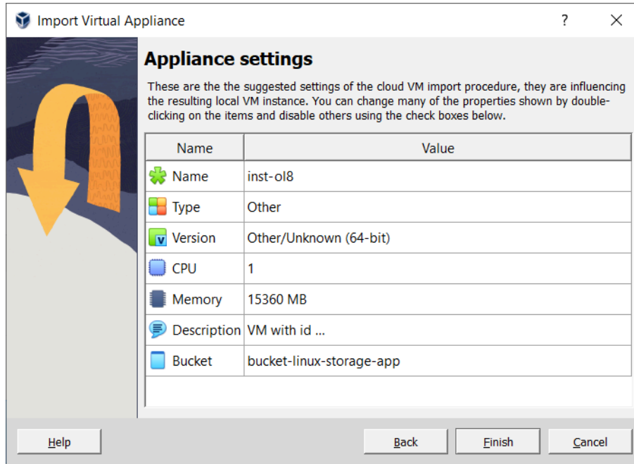
Figure 9: Import Cloud Instance Wizard: Appliance Settings
