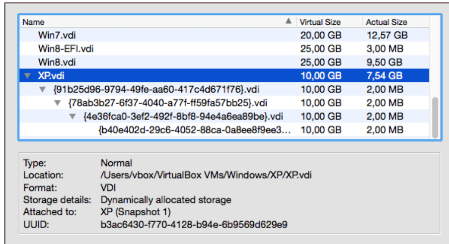
Figure 16: Differencing Images, Shown in Virtual Media Manager
