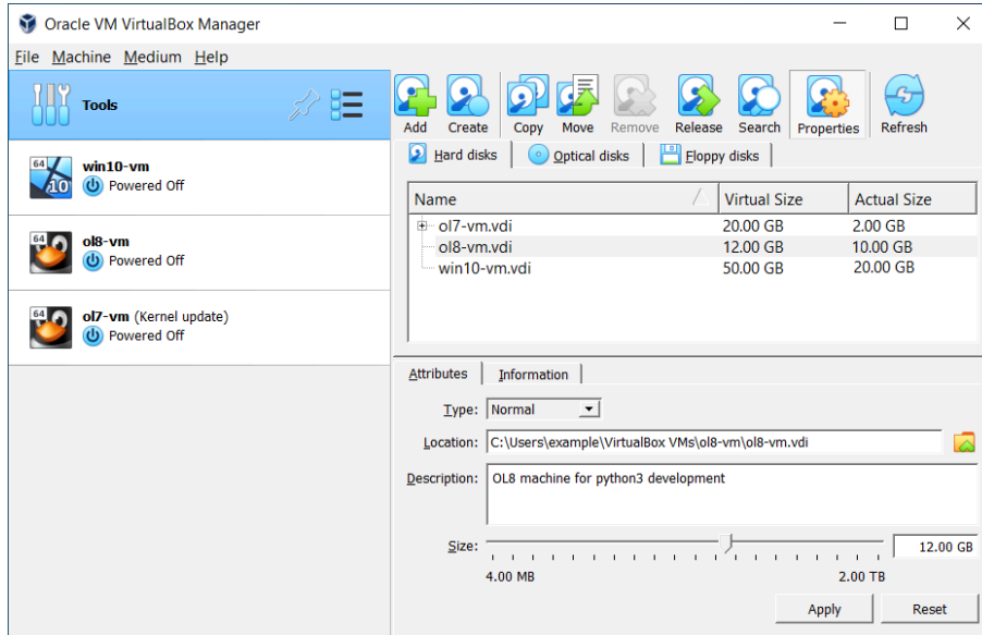
Figure 14: The Virtual Media Manager, Showing Hard Disk Images
