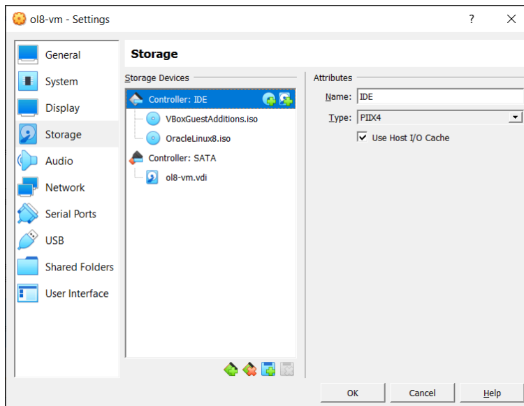
Figure 10: Storage Settings for a Virtual Machine
